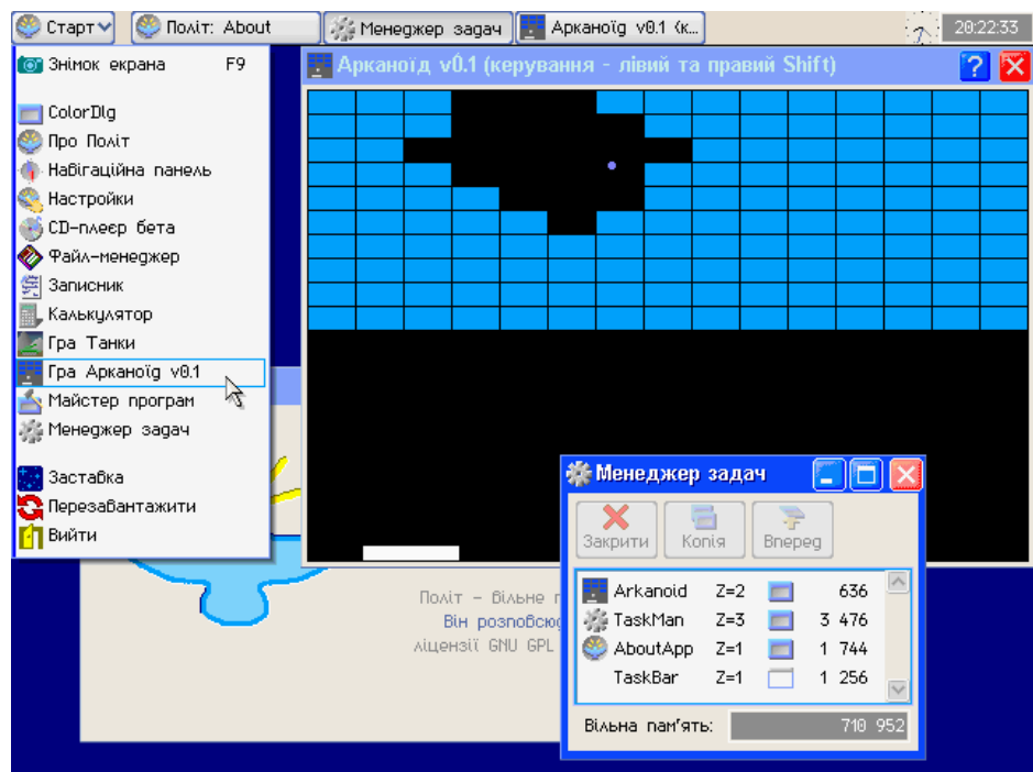
24.06.2003 Windows XP menu style , soft shadow from the menu. Arkanoid game started . A task manager that shows the memory occupied by each program and the free memory. "Semi-transparent" view of unavailable icons.
